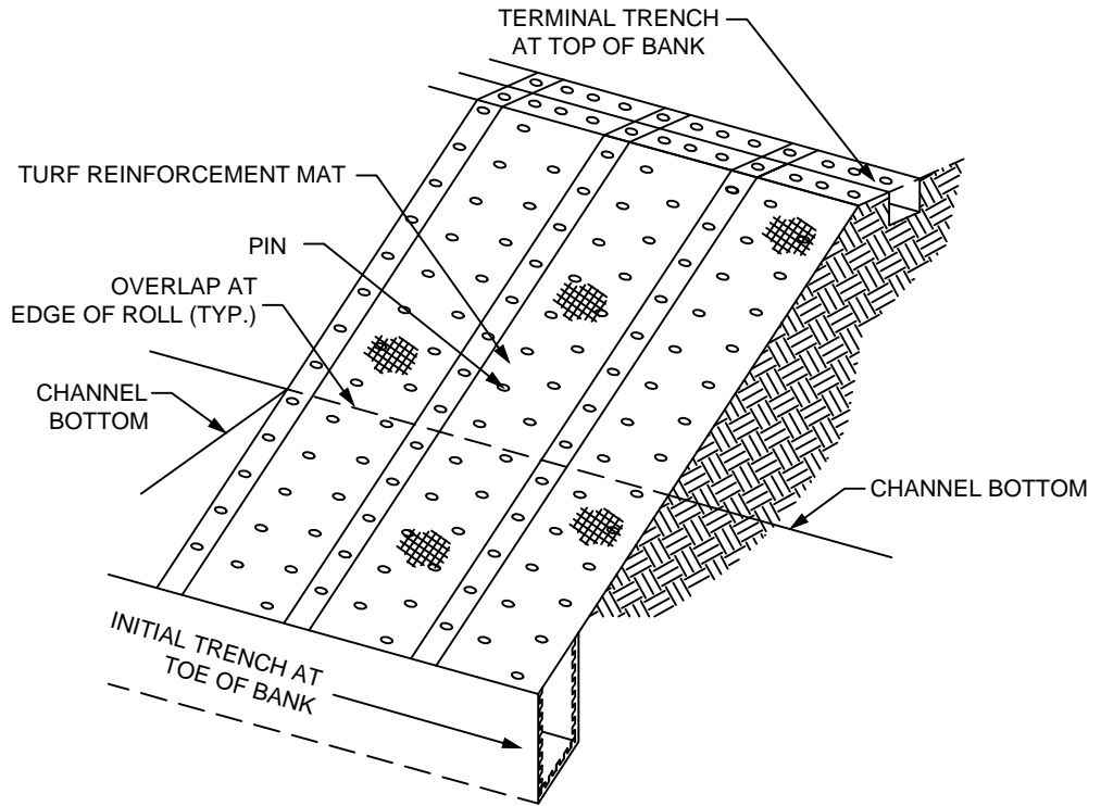
OVERVIEW OF TURF REINFORCEMENT MAT ON A CHANNEL BANK
