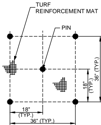
PIN PATTERN DETAIL
